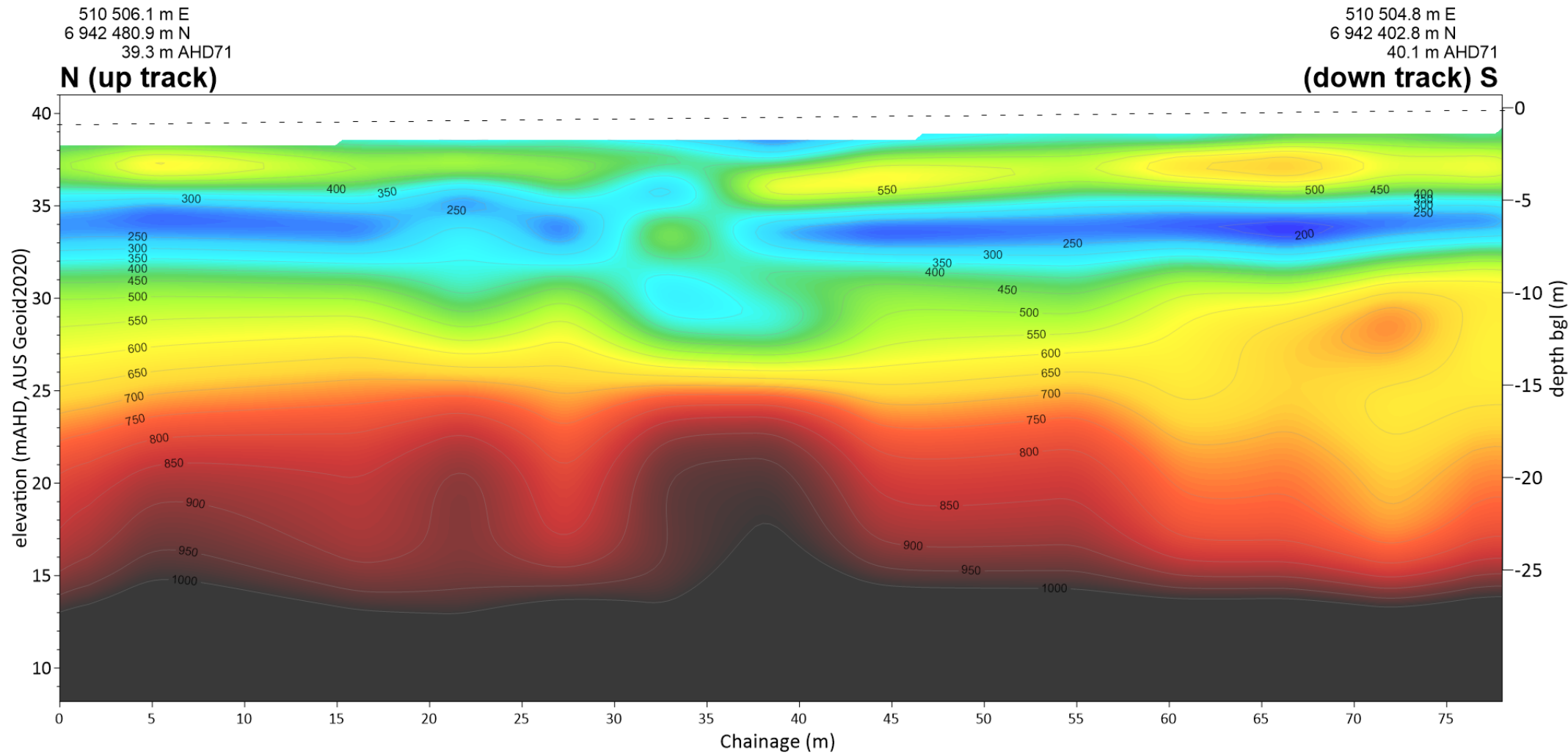
Seismic Line MASW AU-GP 133
